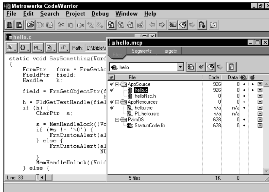
Figure 3-1: The CodeWarrior IDE
