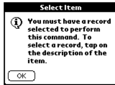
Figure 9-7: The built-in To Do application displays this dialog box when the user tries to use the Record ⇄ Delete Item menu command without selecting an item.
