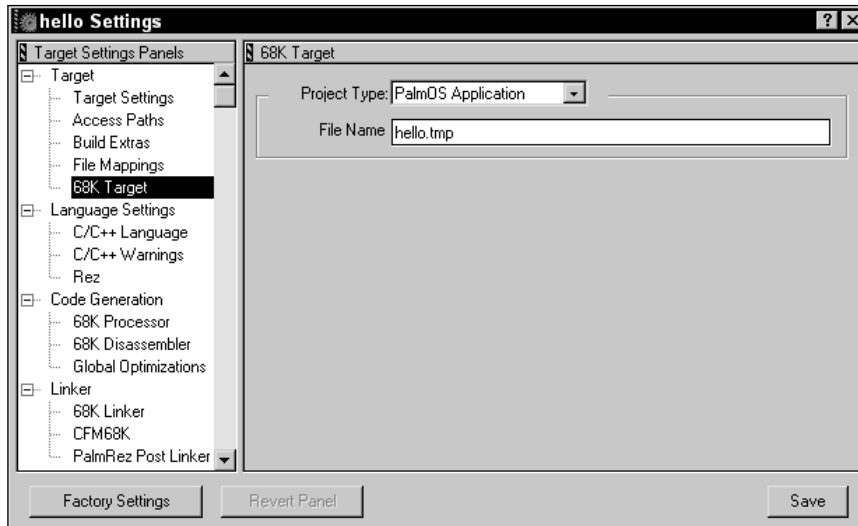
Figure 3-9: The 68K Target panel
