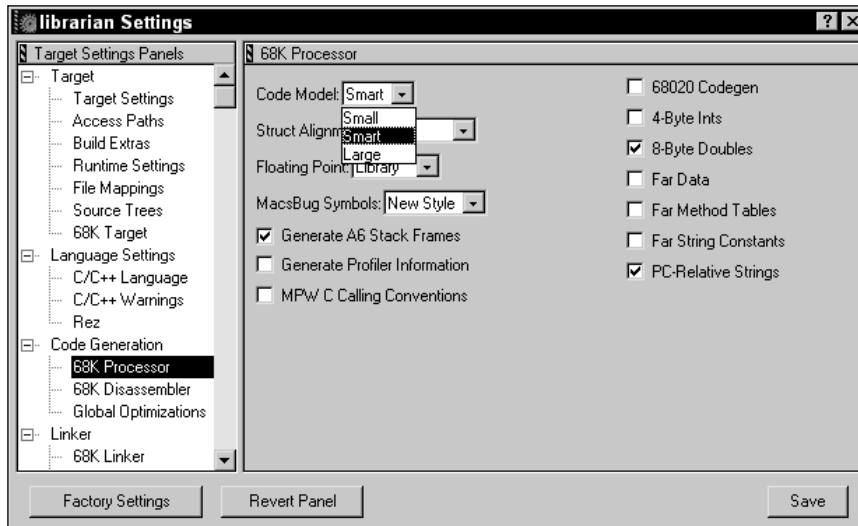
Figure 20-2: Enabling the Smart code model in the Target Settings Panel
