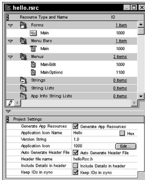
Figure 6-6: Constructor's project window
