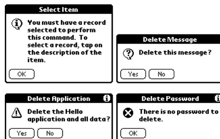
Figure 2-3: Alert dialogs come in four flavors (clockwise from upper left): information, confirmation, error, and warning.
