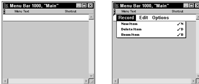
Figure 8-1: The menu bar editor window, as it appears when it first opens (left) and after adding menus (right)
