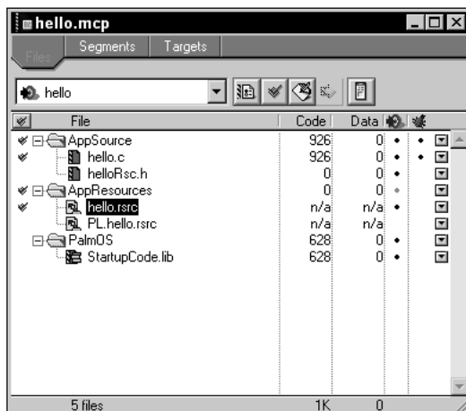
Figure 3-4: The project window's File view
