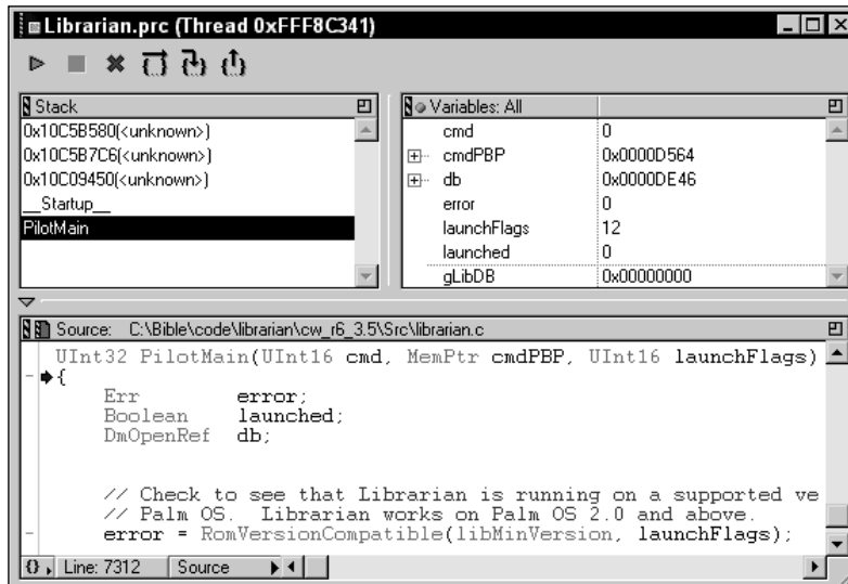
Figure 5-23: CodeWarrior's debugging window
