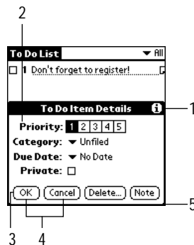
Figure 6-4: Dialog box layout from the To Do List application
