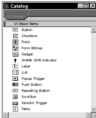
Figure 6-16: The Catalog window
