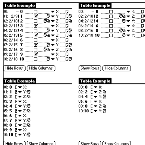
Figure 11-2: The Table Example program demonstrates hiding rows and columns. Clockwise from upper left: nothing hidden, rows hidden, both rows and columns hidden, columns hidden.
