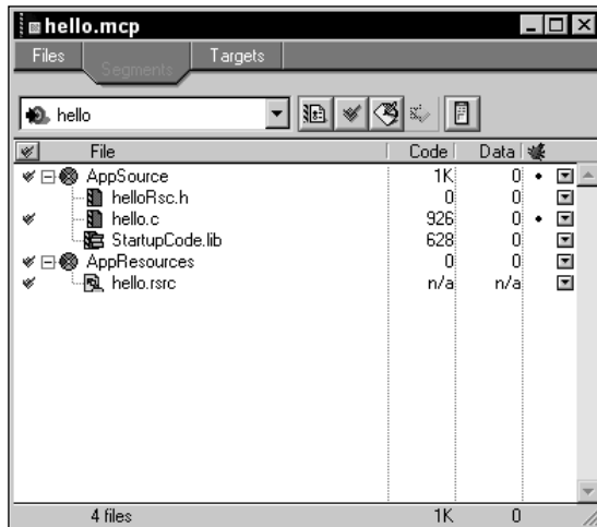
Figure 3-5: The project window's Segment view
