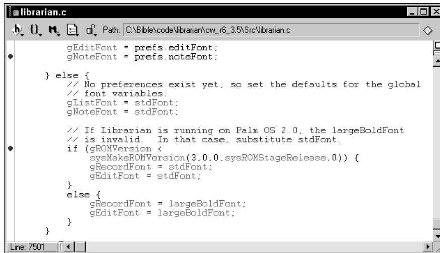
Figure 5-19: A CodeWarrior code window with the breakpoint column displayed
