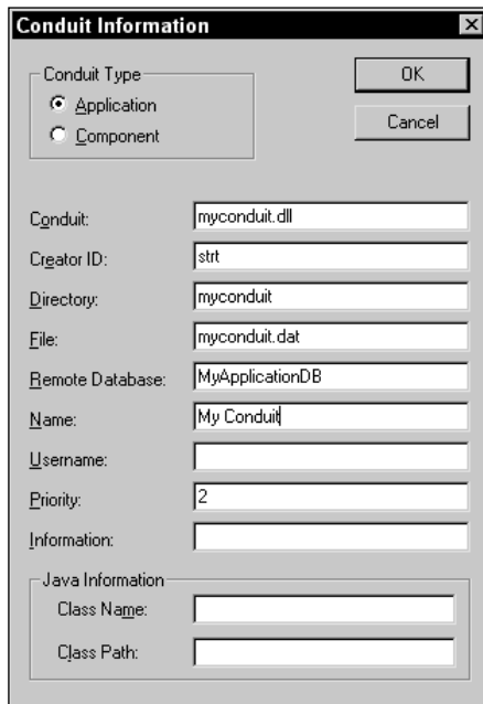
Figure 17-4: The Conduit Configuration tool's Conduit Information dialog box
