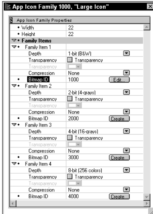
Figure 6-15: The app icon family editor window
