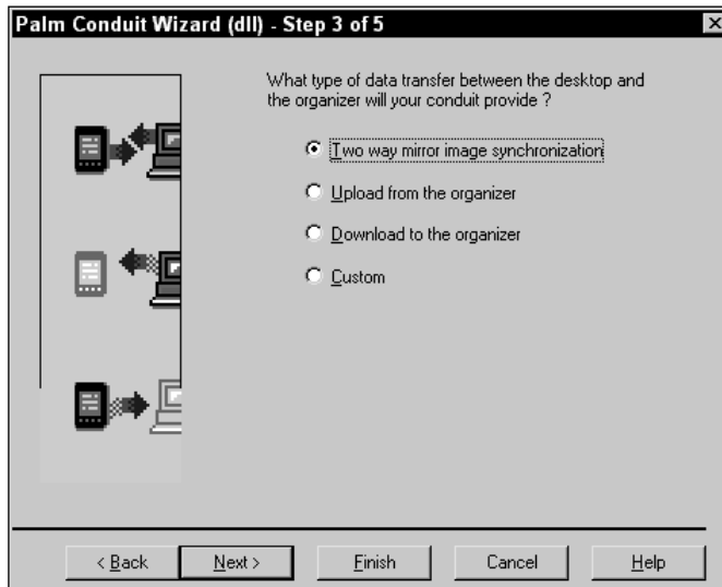
Figure 18-4: Conduit Wizard Step 3: data transfer selection
