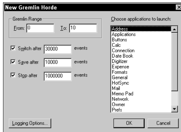
Figure 5-12: The New Gremlin Horde dialog in POSE
