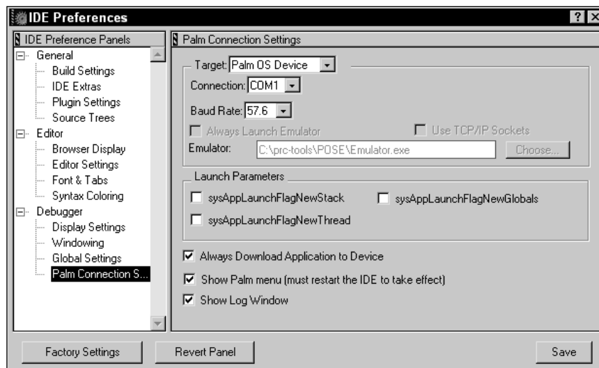
Figure 5-21: The CodeWarrior IDE Preferences dialog, set up to connect to an actual Palm OS handheld
