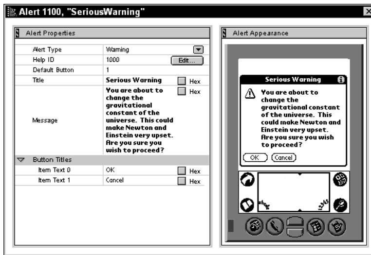
Figure 6-11: The alert editor window
