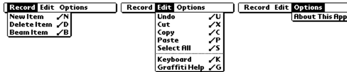
Figure 8-2: The menu bar generated from Menus.r
