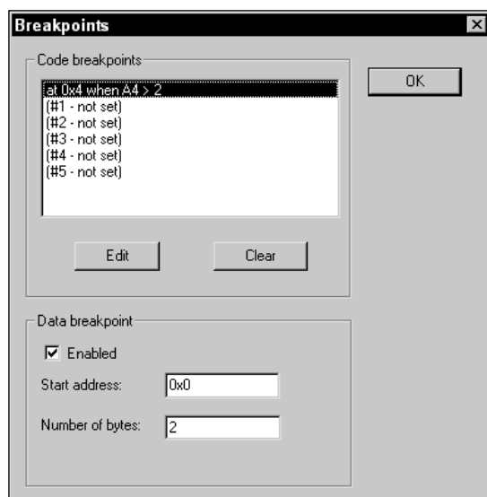
Figure 5-10: The Breakpoints dialog in POSE
