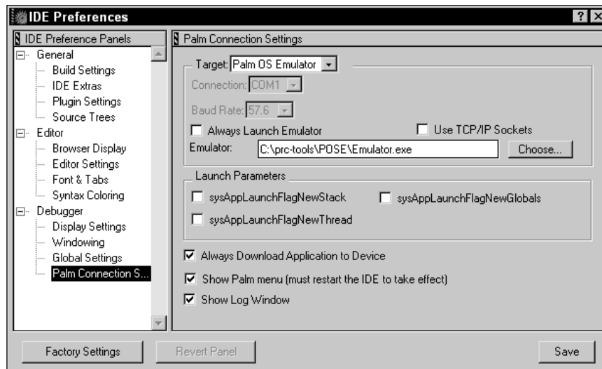
Figure 5-20: The CodeWarrior IDE Preferences dialog, set up to connect to POSE for debugging
