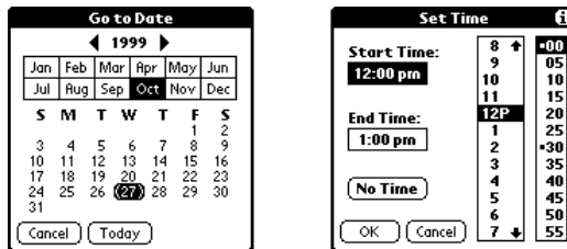
Figure 9-4: The Palm OS built-in date (left) and time (right) picker dialog boxes
