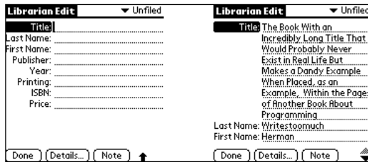
Figure 11-6: The Edit view in Librarian must handle the extremes of fewer data fields than table rows (left) and fewer table rows than data fields (right).
