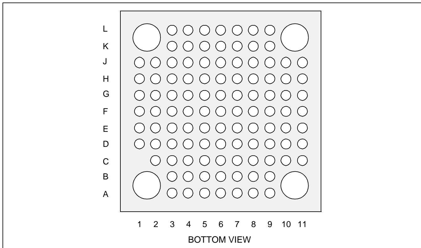
Figure 4-2: Pinout Diagram - CFLGA - 104pin (SID13706B00A)
