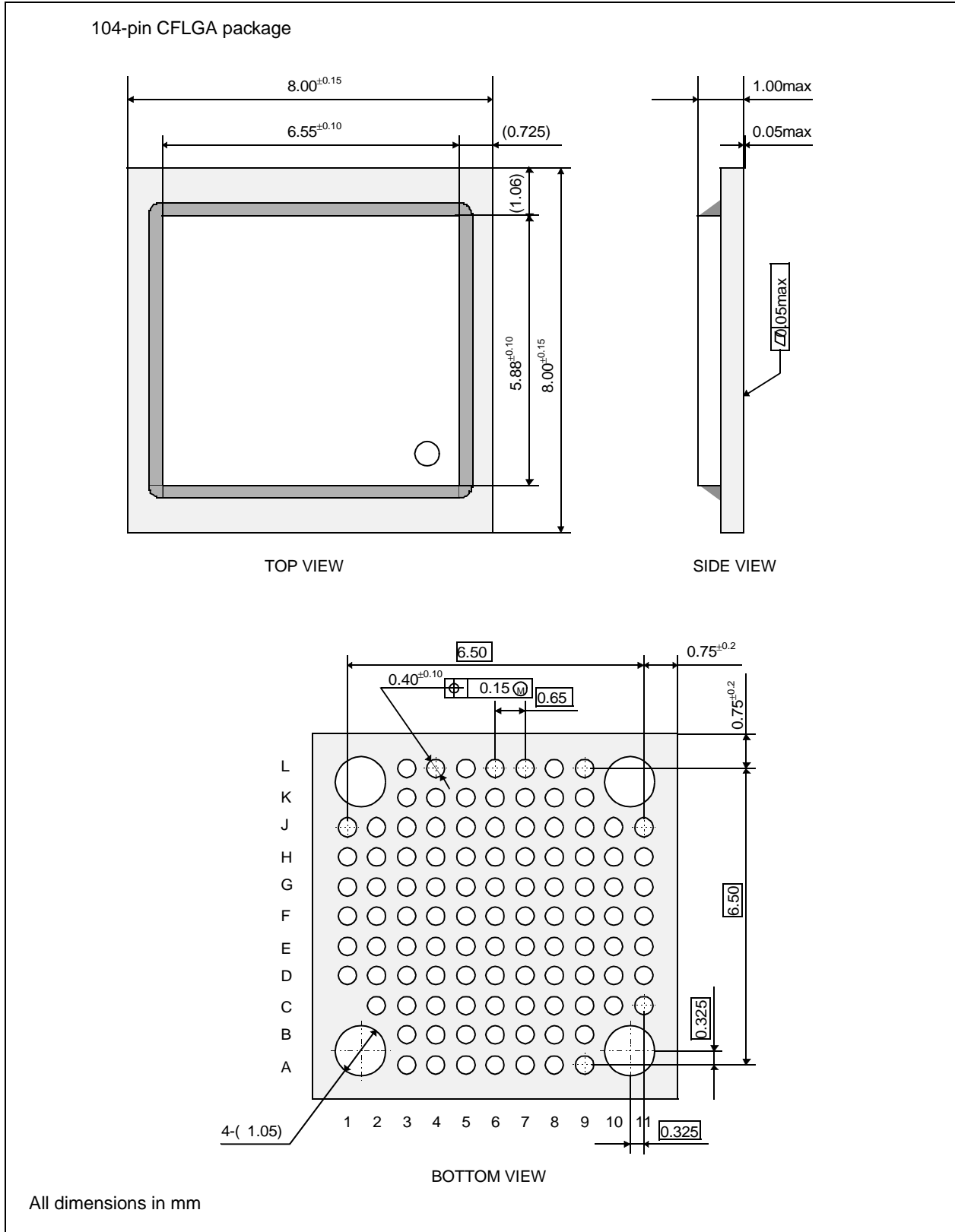
Figure 16-2: Mechanical Data 104pin CFLGA (SID13706B00A)
